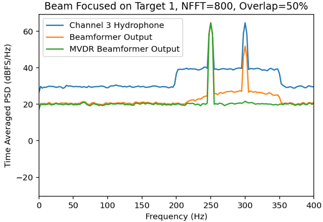
Figure 7. Welch's method graph comparison between all methods for artificial data
