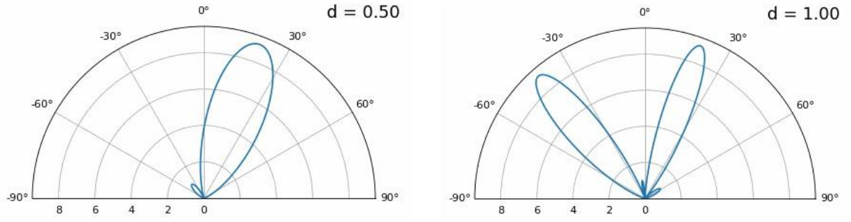
Figure 1. (left) Beamforming without spatial aliasing, (right) grating lobes becoming introduced [5]
