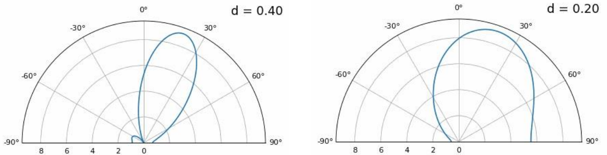
Figure 2. The effect of spacing on angular resolution [5]
