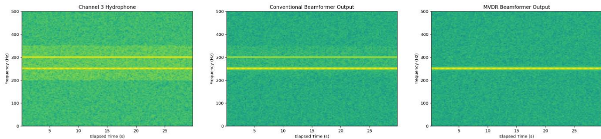
Figure 8. Spectrogram display comparison between all methods for artificial data
